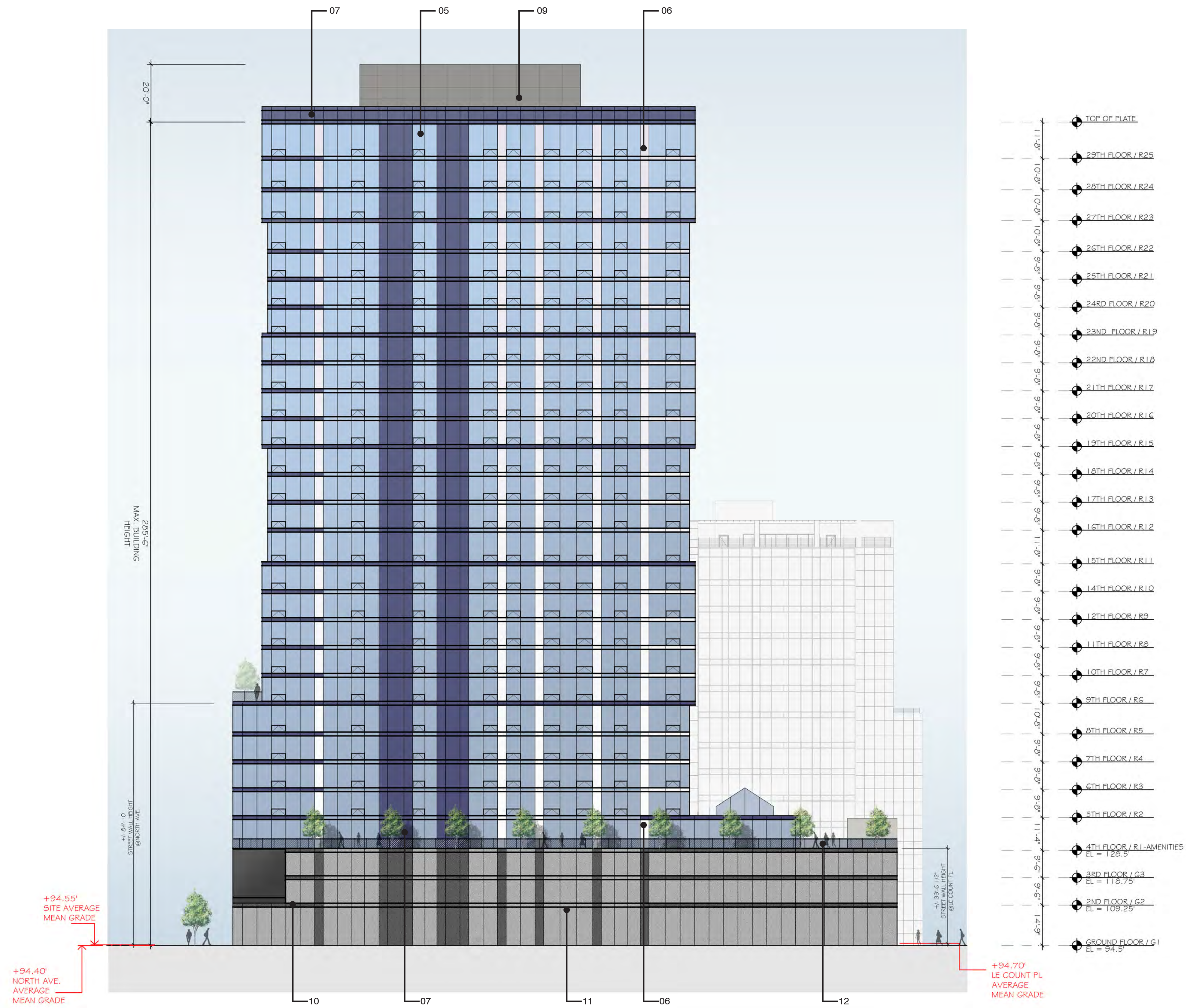
BUILDING ELEVATION 2
